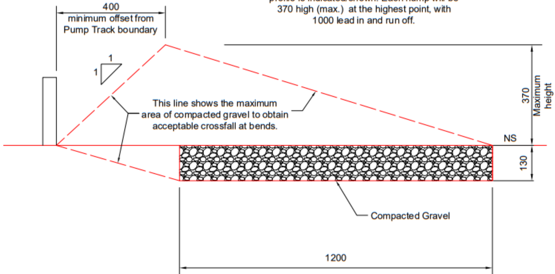
EAST DEVONPORT PRIMARY SCHOOL PUMP TRACK - SECTION A-A Sheet 2 of 2
