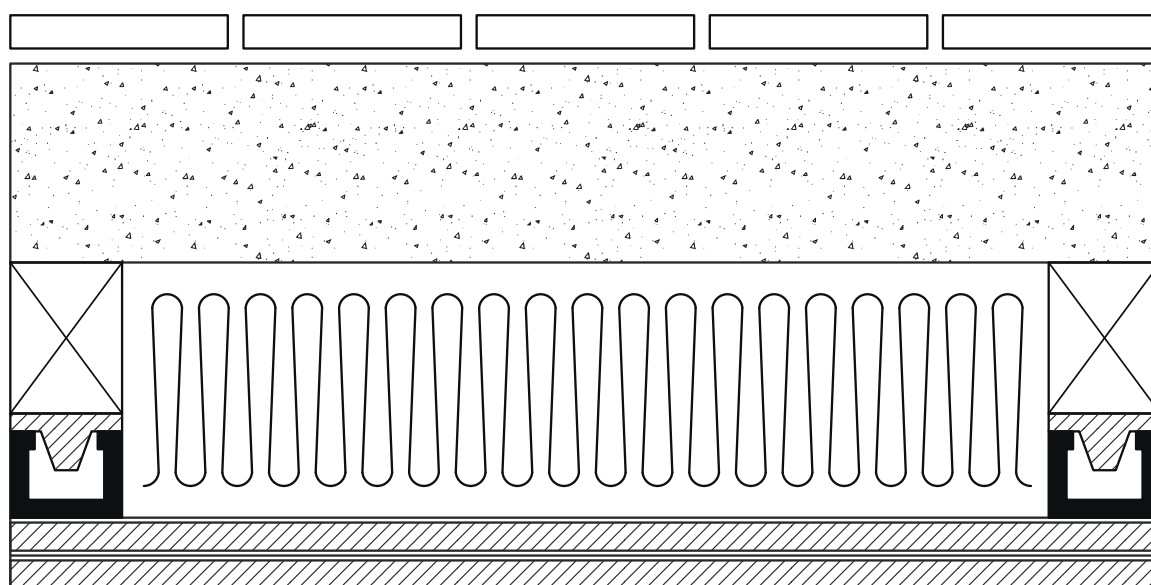
Figure S28C9: 75 mm thick autoclaved aerated concrete floor panel
