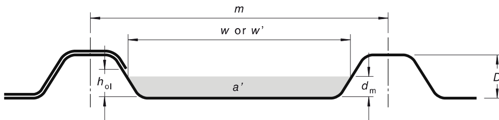
FIGURE D1 ROOFING PROFILE WITH NO ANTI-CAPILLARY FEATURE
