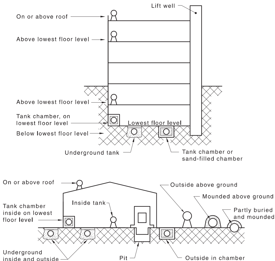
FIGURE 5.1 ILLUSTRATIONS OF TERMS RELATING TO TANK LOCATIONS
