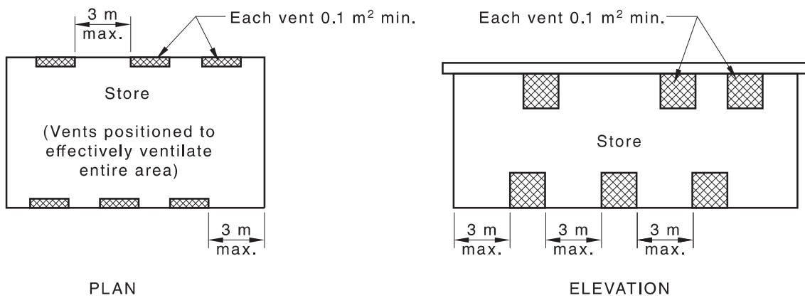
(d) A Store having vents in one pair of opposite external walls
