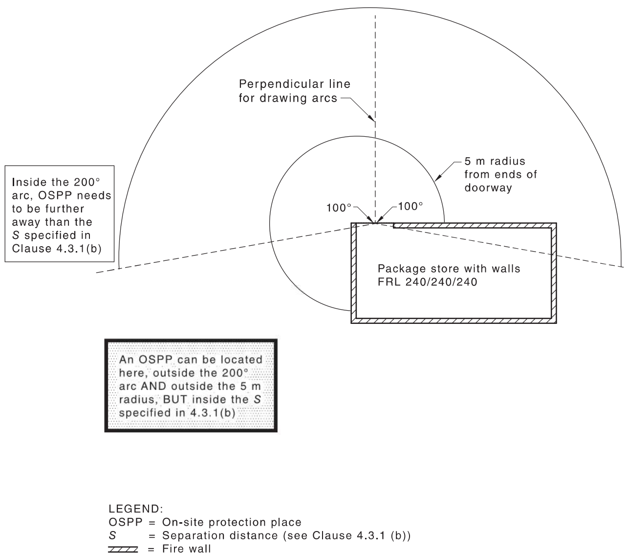
FIGURE 4.4 USE OF NON-FIRE-RATED DOORS
