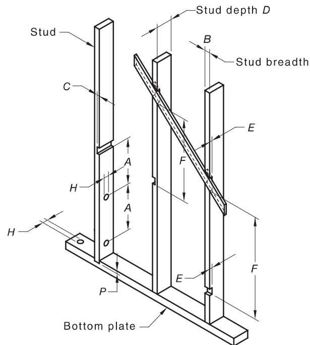
Figure 5.5.2.1(A) — Notching of wall studs
