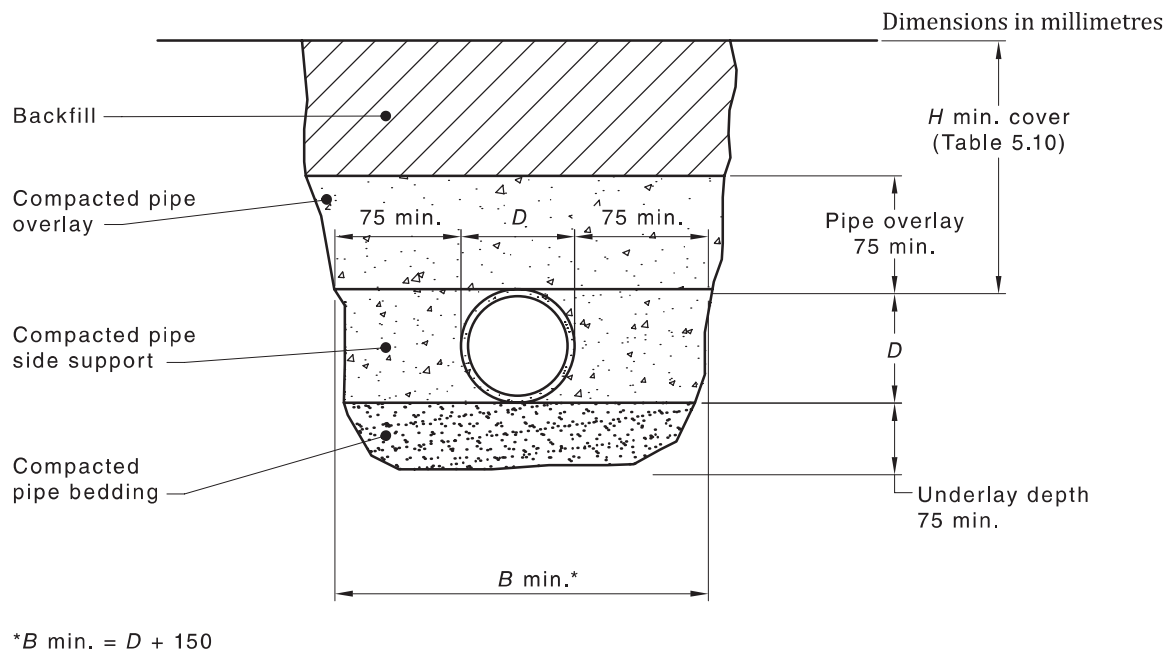
Figure 5.11 — Typical installation in a trench
