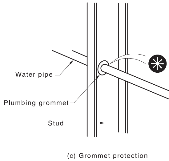
Figure 5.5.2.1(D) — Installation and fixing of services
