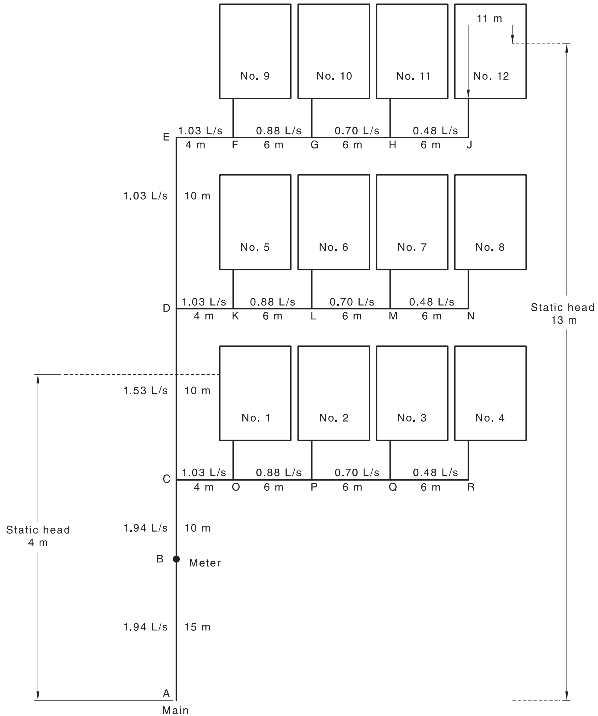
Step 1 Sketch of installation
