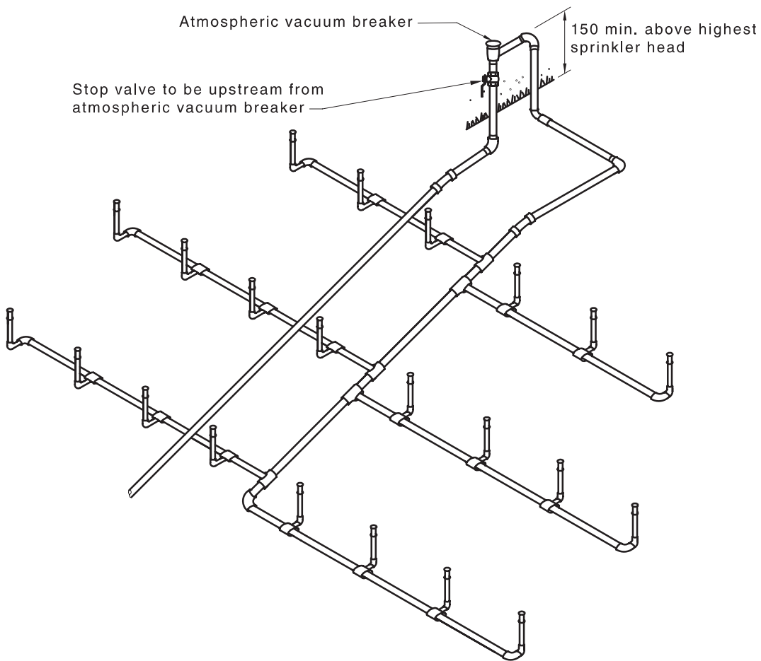
(ii) Hillside system using atmospheric vacuum breaker
