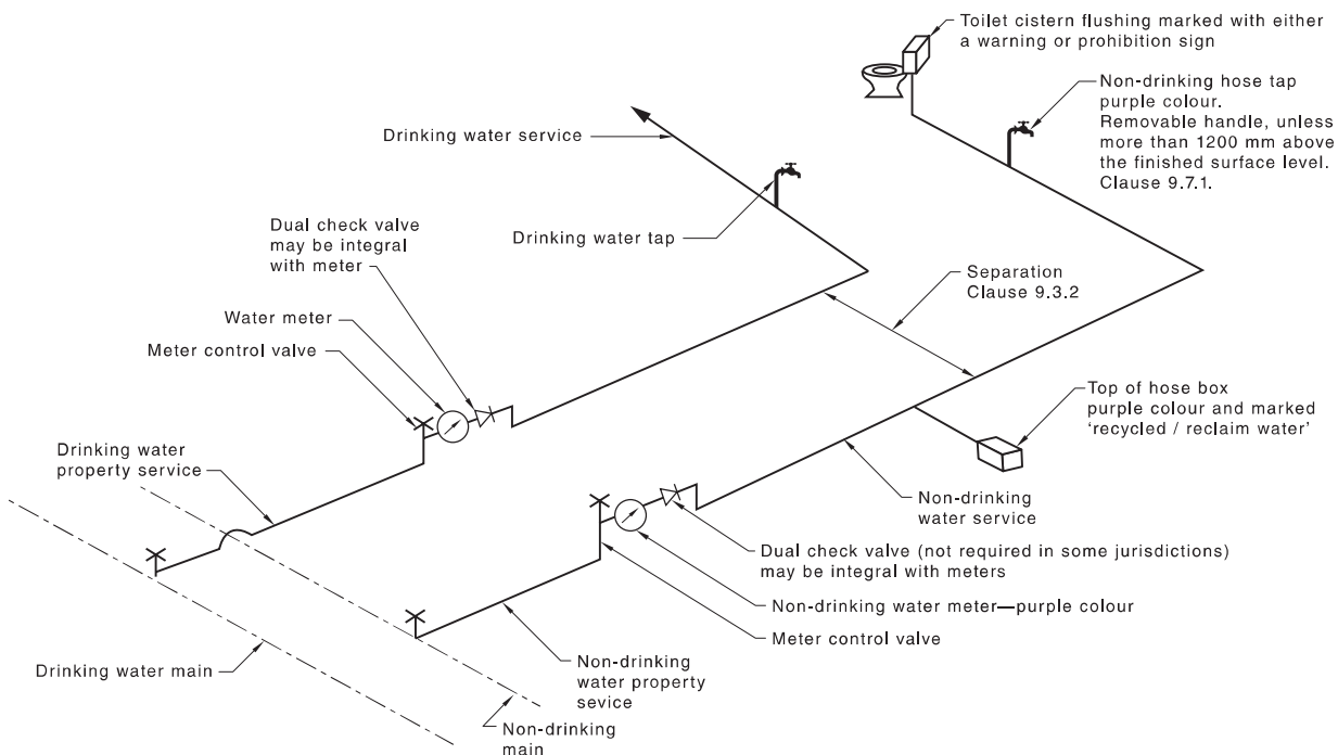
Figure 9.1 — Typical non-drinking water installation from a reticulated non-drinking water system
