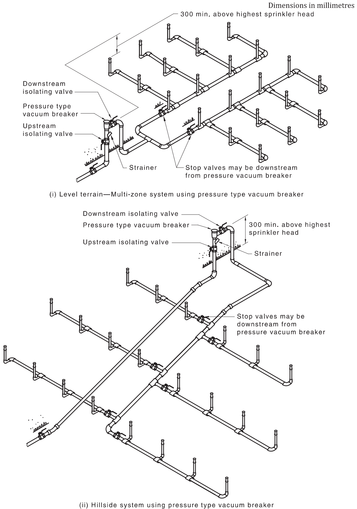
Figure 7.2(D) — Type C system — Testable devices — No back-pressure
