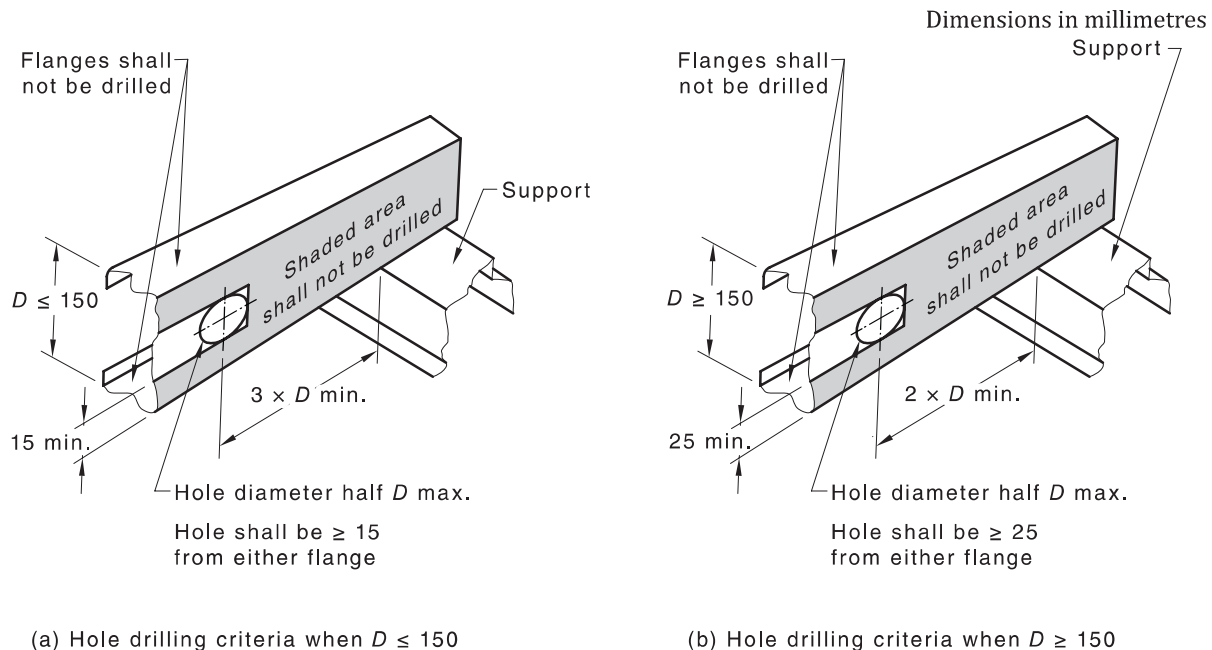
Figure 5.5.2.1(E) — Penetrations to steel floor joists
