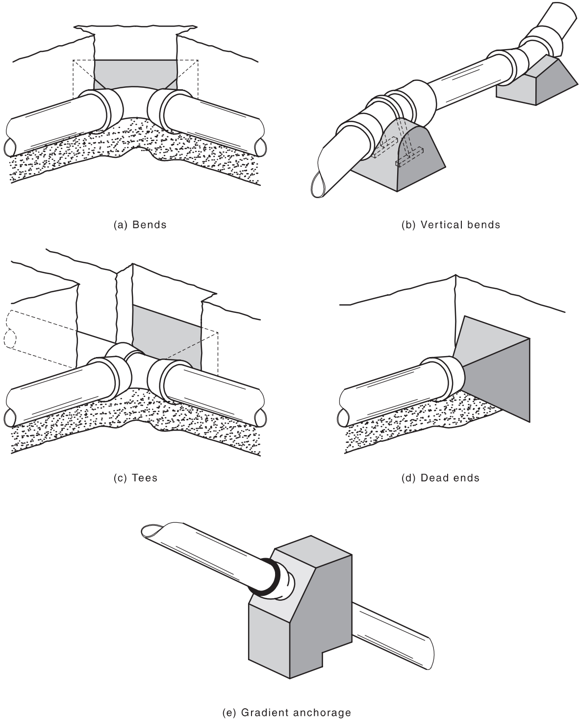
Figure 5.9.2 — Typical locations of thrust blocks
