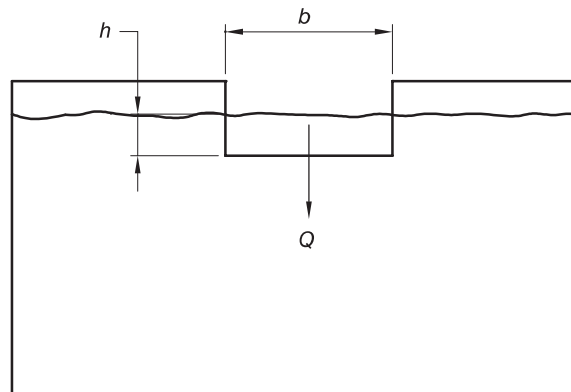
Figure 8.4.4.1(B) — Rate of outflow from type 2 overflow (piped) vertical outlet storage tanks
