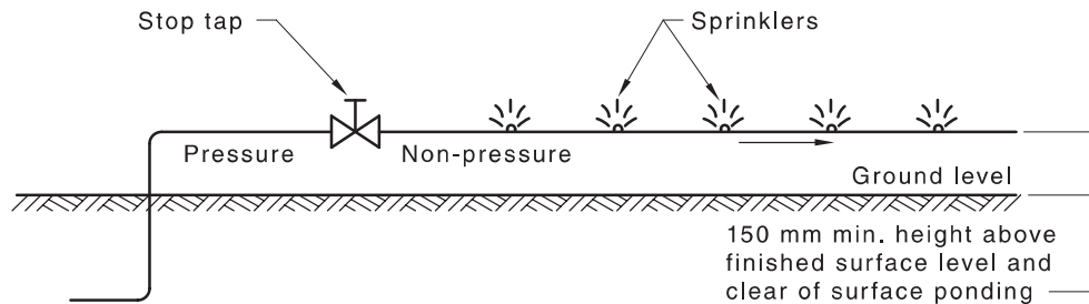
Figure 7.2(A) — Type A system — No backflow prevention required
