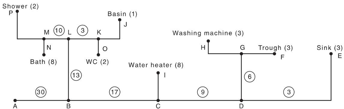
Figure D.3 — Sketch of installation
