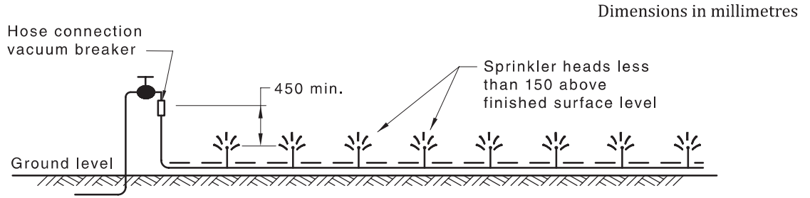
(iii) System using hose connection vacuum breaker
