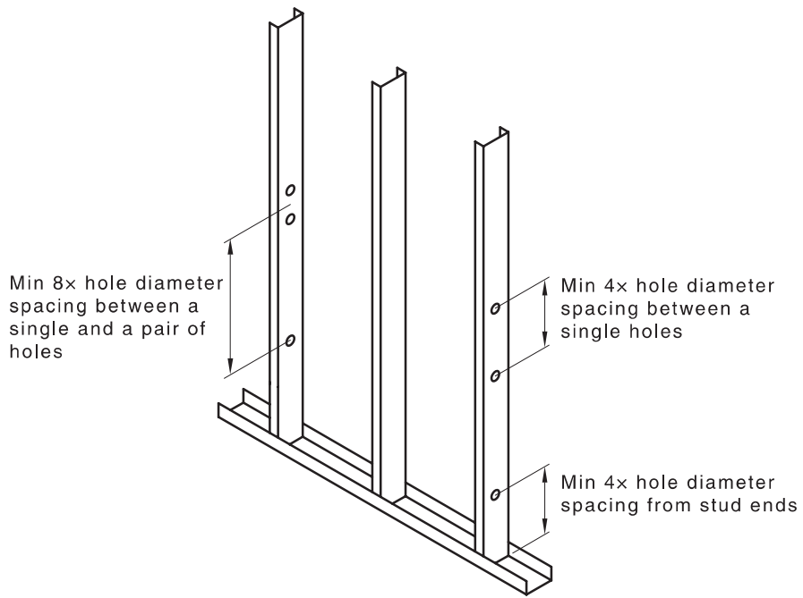
Figure 5.5.2.1(C) — Hole spacing in metal wall framework
