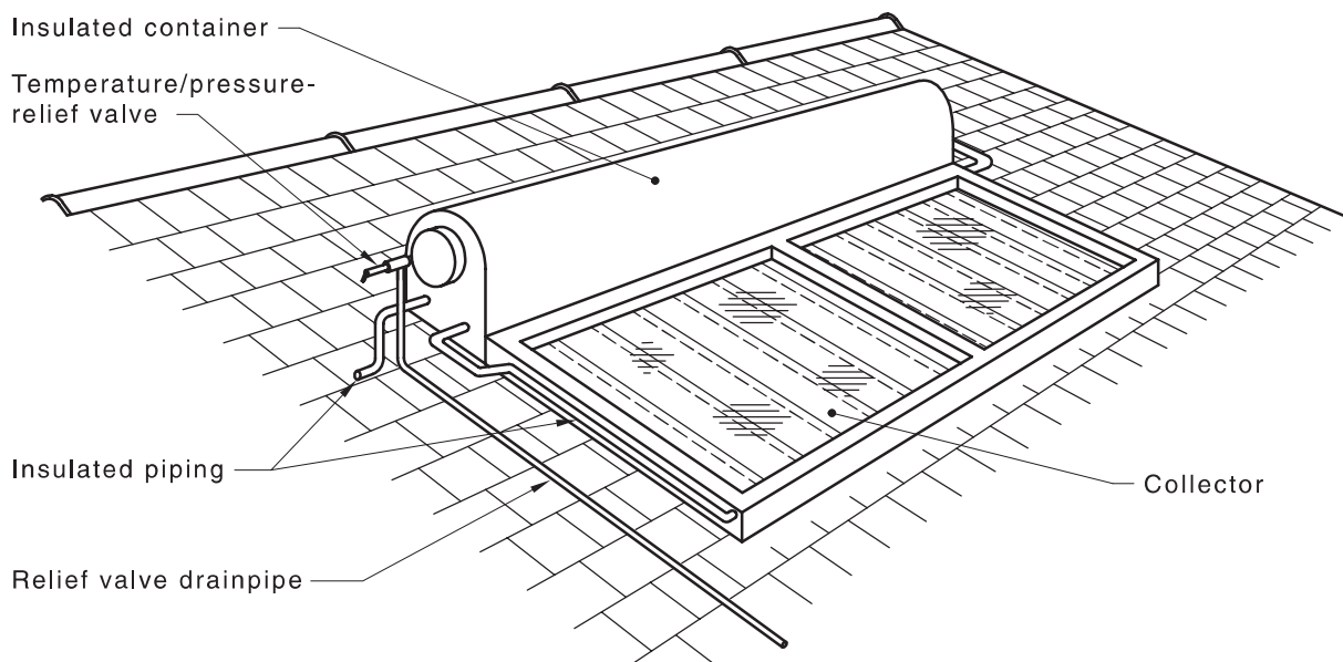
Figure F.2.1 — “With pitch” installation
