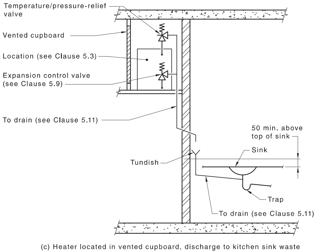
Figure 5.11.3(A) — Typical relief drainage
