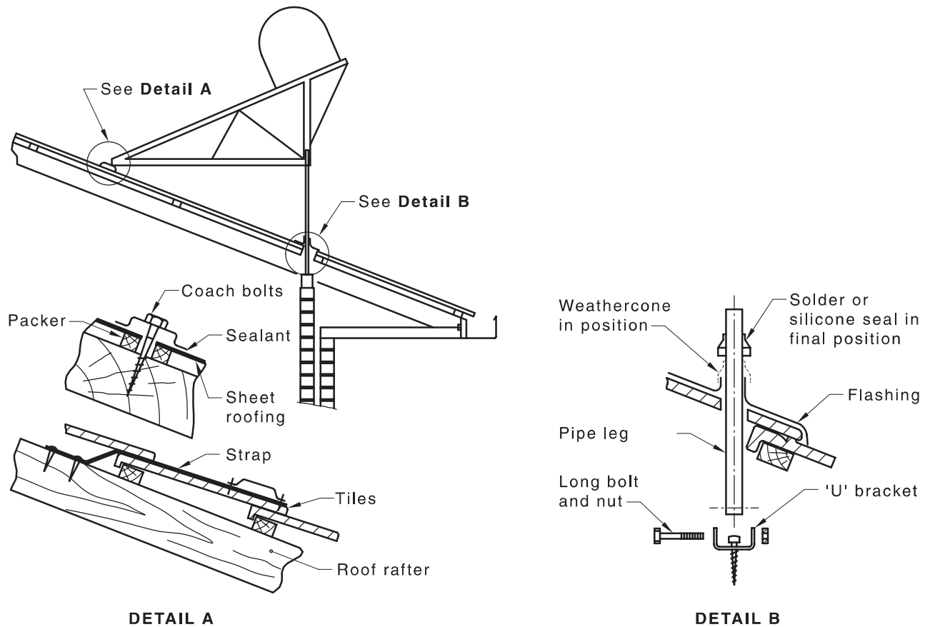
Figure F.2.2 — "Against pitch" installation
