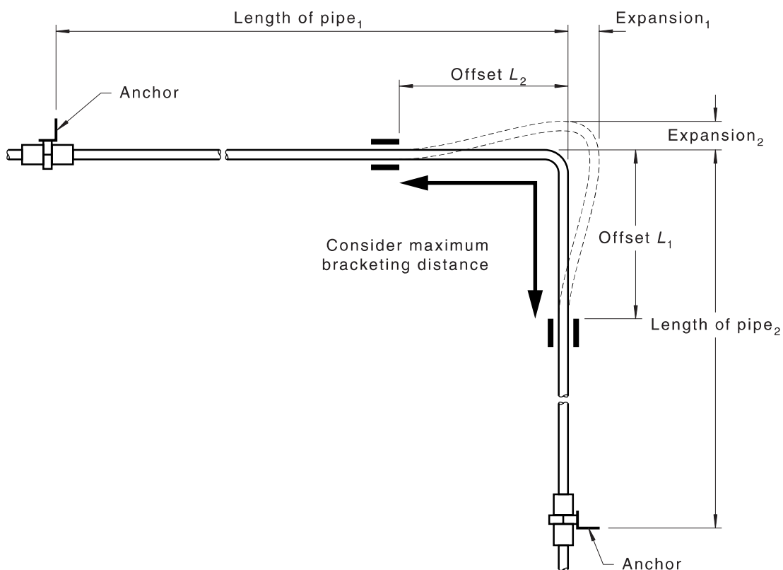
Figure N.6 — Offset to accommodate expansion from two directions
