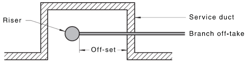
a) Straight off-set in duct — Plan view
