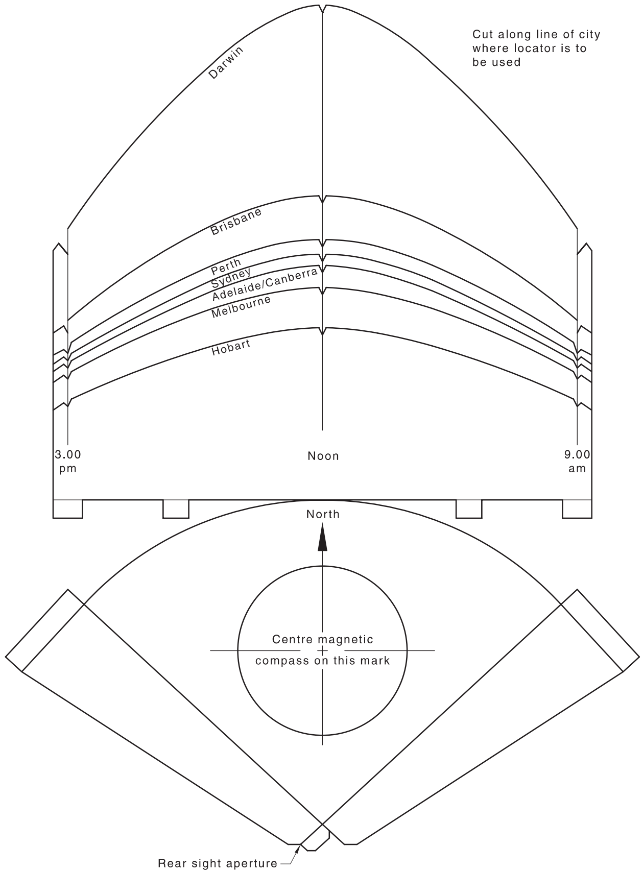
Figure H.2(A) — Mid-winter solar altitude sight (Australia)
