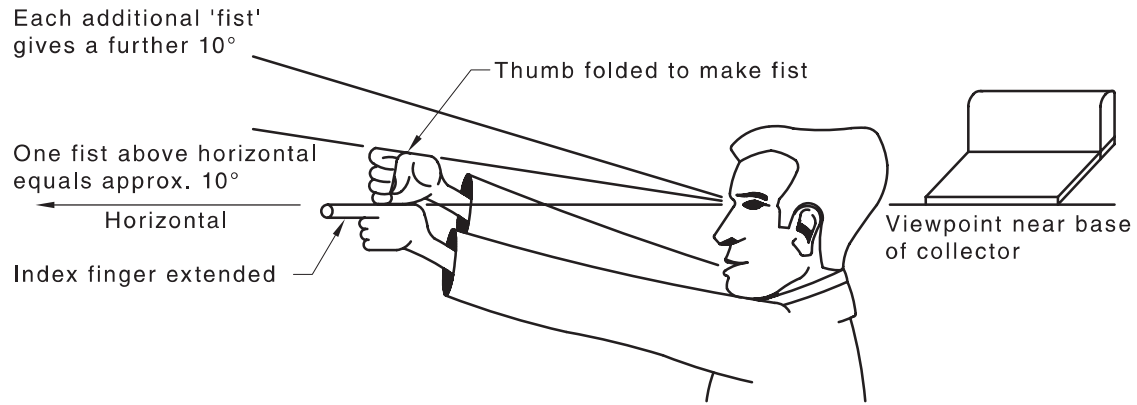
Figure H.3 — “Fist” method of estimating solar altitude
