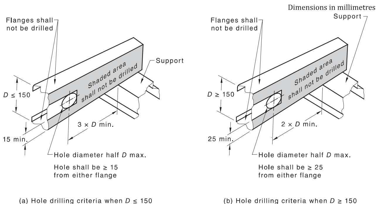
Figure 4.6.1.1(D) — Penetrations to steel floor joist
