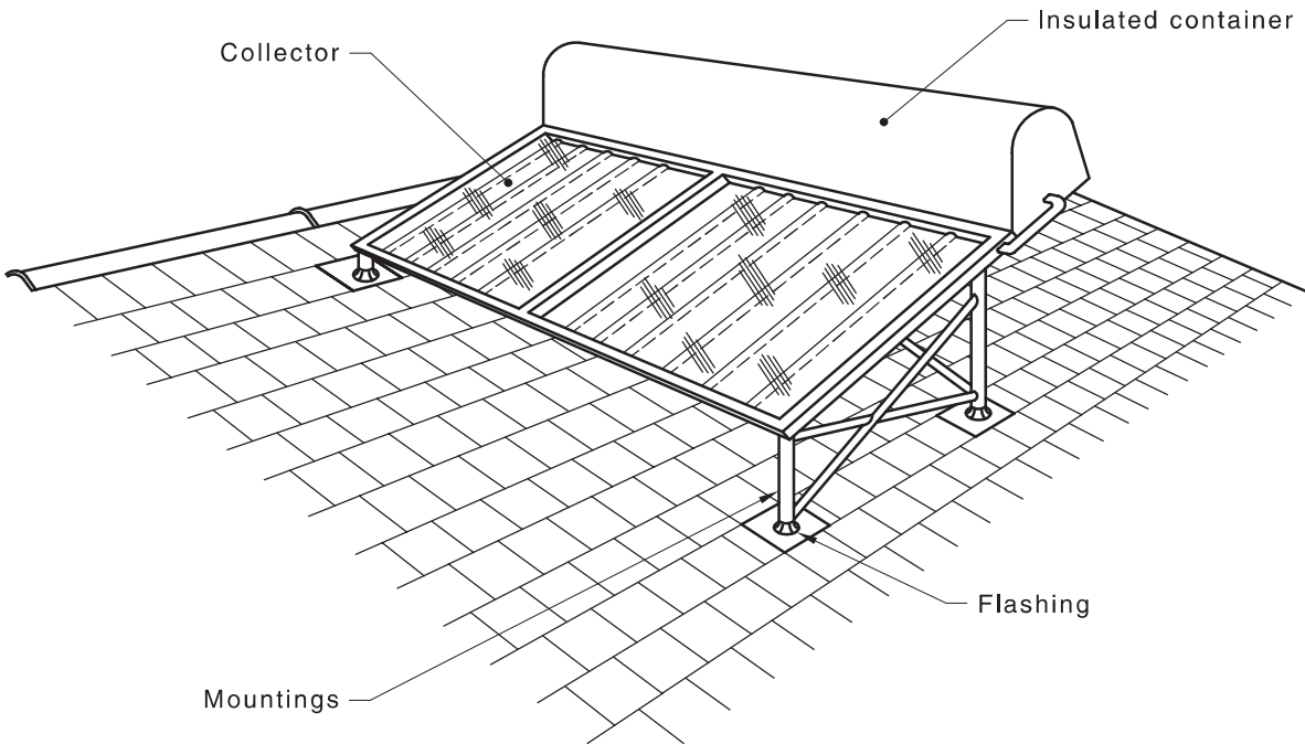
Figure F.2.3 — “Cross-pitch” installation
