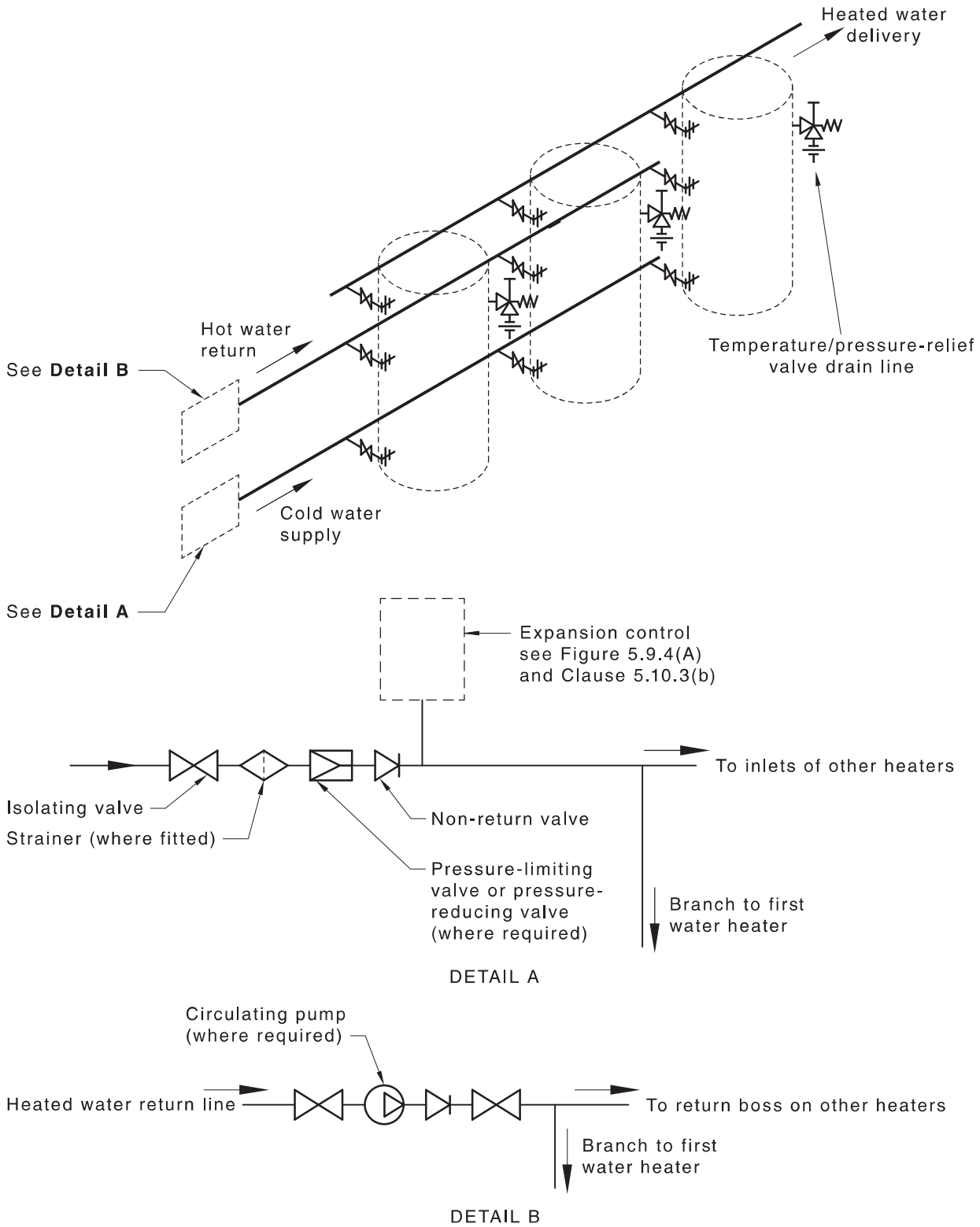
Figure 5.10.2(B) — Typical alternative arrangement of heated water return line for circulating heated water service
