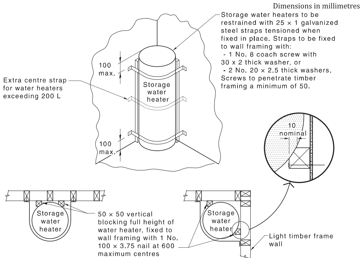
Figure 5.5.4 — Typical arrangement for seismic restraint of storage water heaters less than 350 L (New Zealand only)
