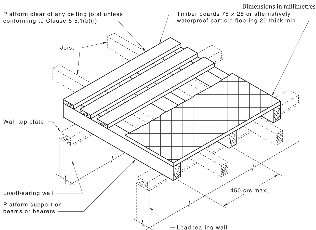
Figure 5.5.3 — Typical construction of a platform
