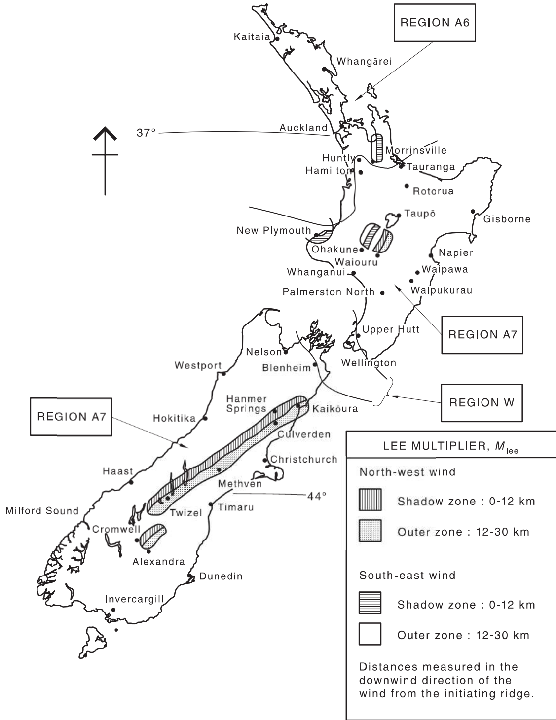
Figure J.2 — New Zealand wind areas
