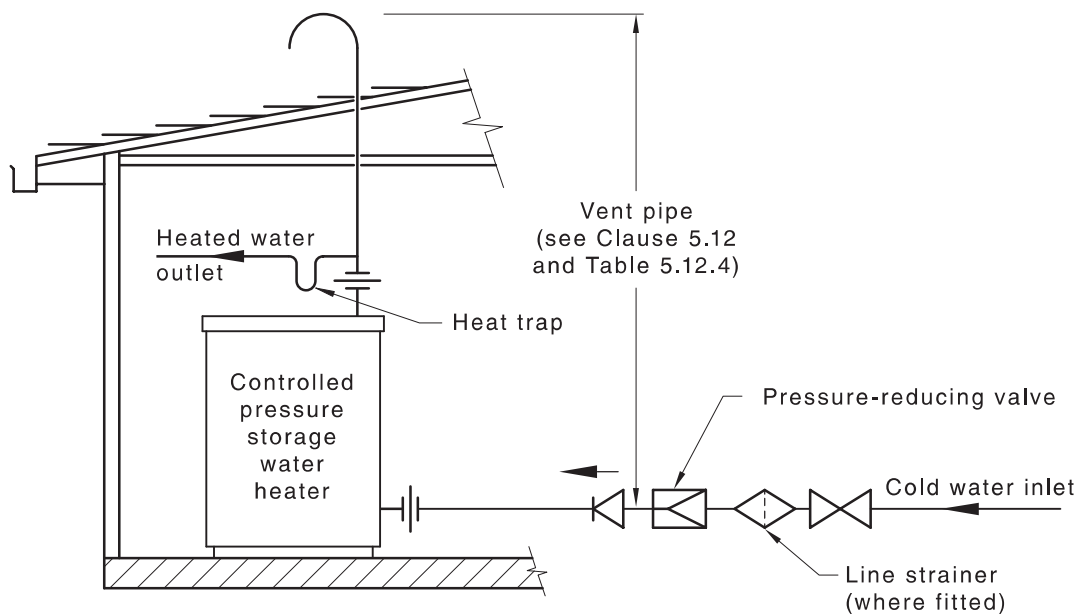
(b) With vent pipe
