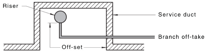
b) Bent off-set in duct — Plan view
