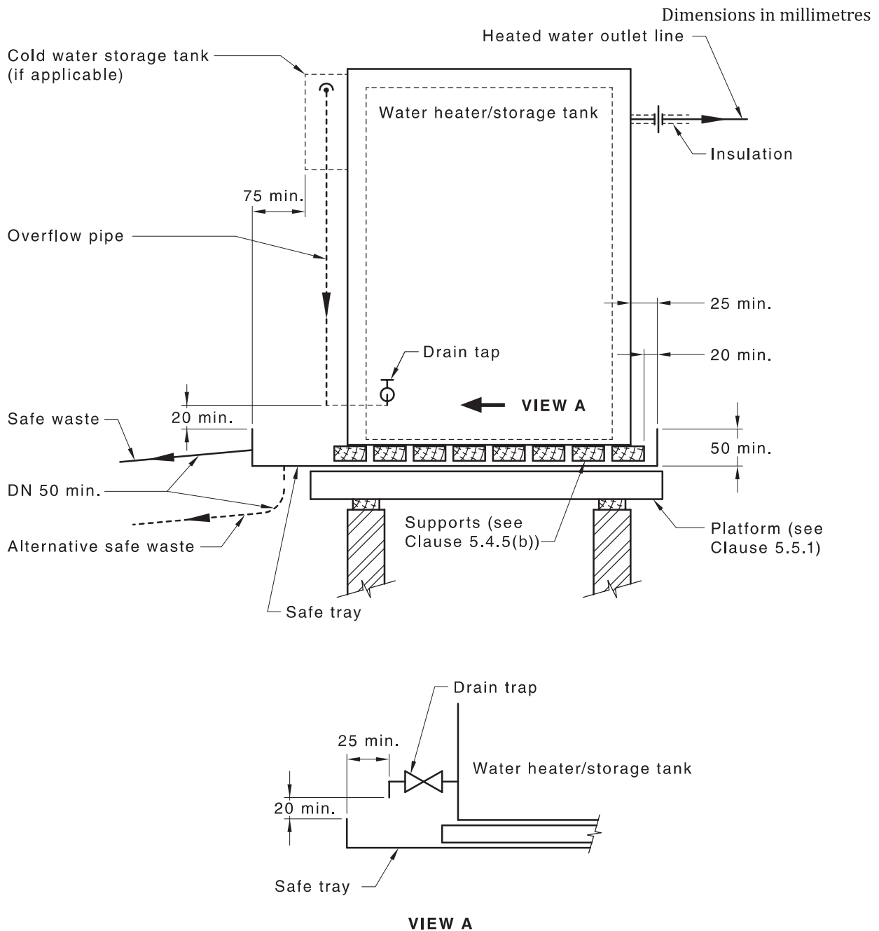
Figure 5.4.5 — Typical installation of a safe tray and position of water heater or cold water storage tank
