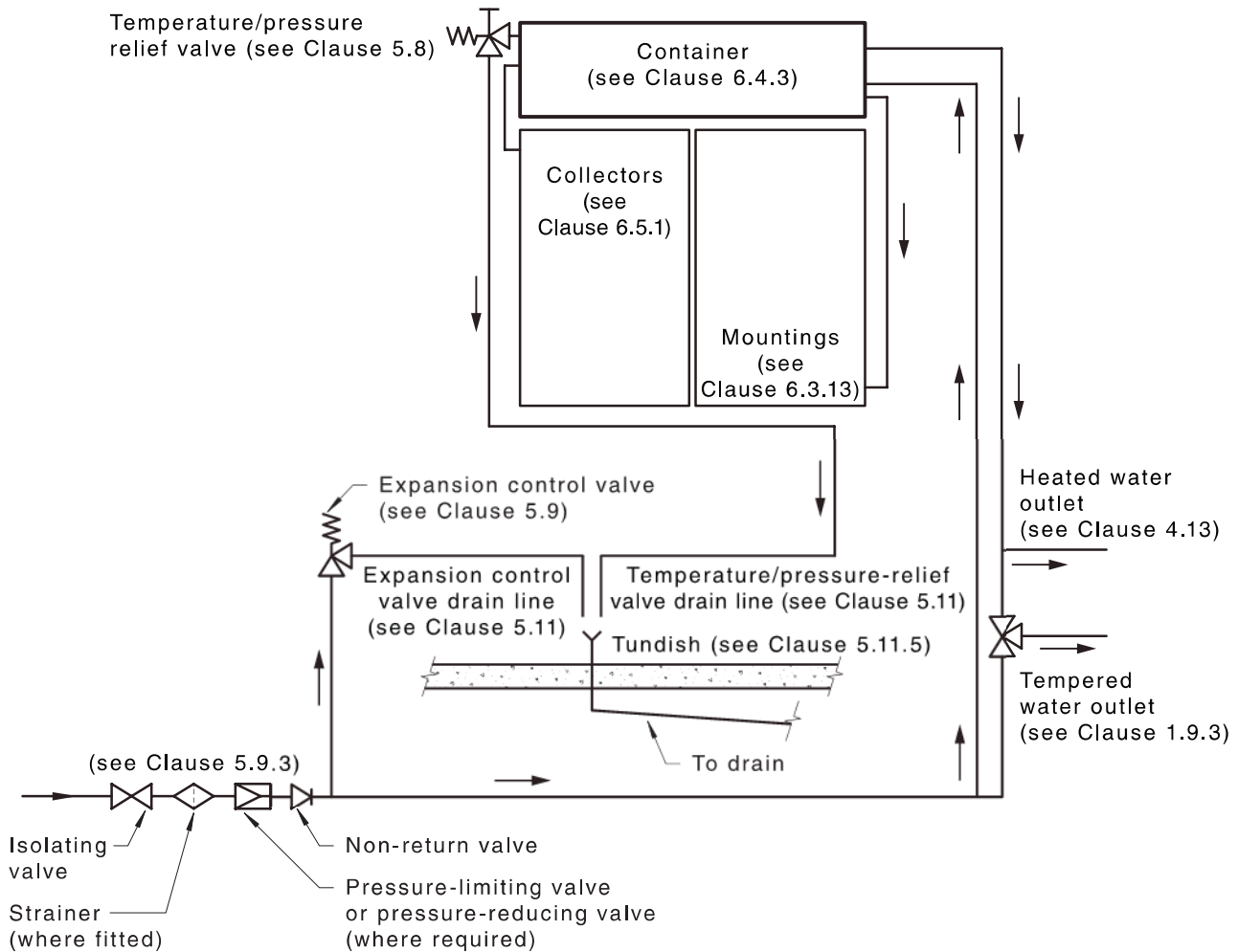
Figure 6.4.3 — Typical installation of close-coupled solar water heater
