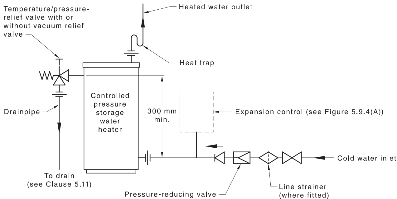
(a) With temperature/pressure-relief and vacuum-relief valves
