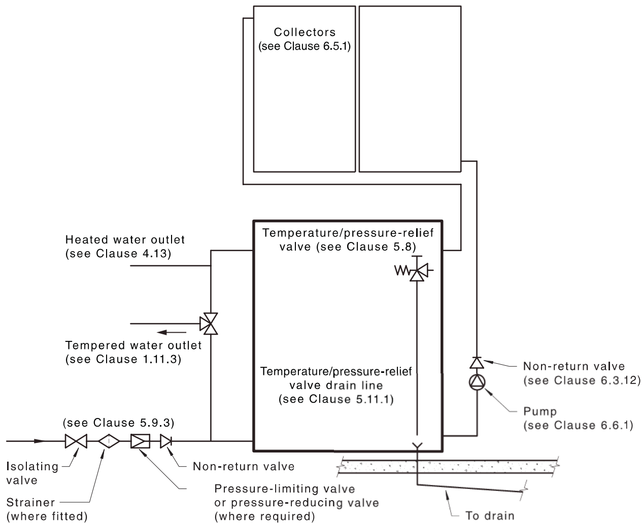
Figure 6.6.1 — Typical installation of a solar water heater with remote container and forced circulation
