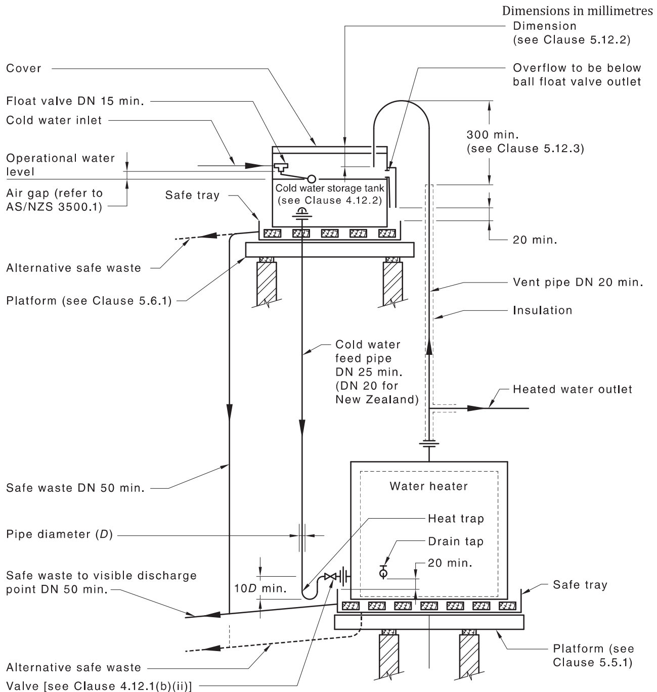
Figure 5.5.1 — Typical installation in roof space of cold water storage tank-fed water heater with separately mounted cold water storage tank
