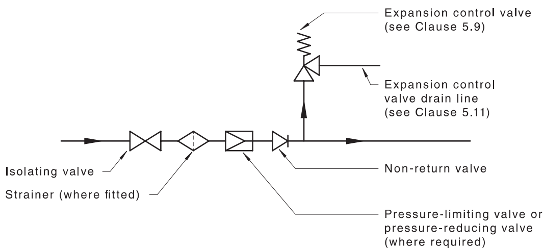
(a) Typical assembly incorporating a pressure-limiting or pressure-reducing valve using expansion control valve
