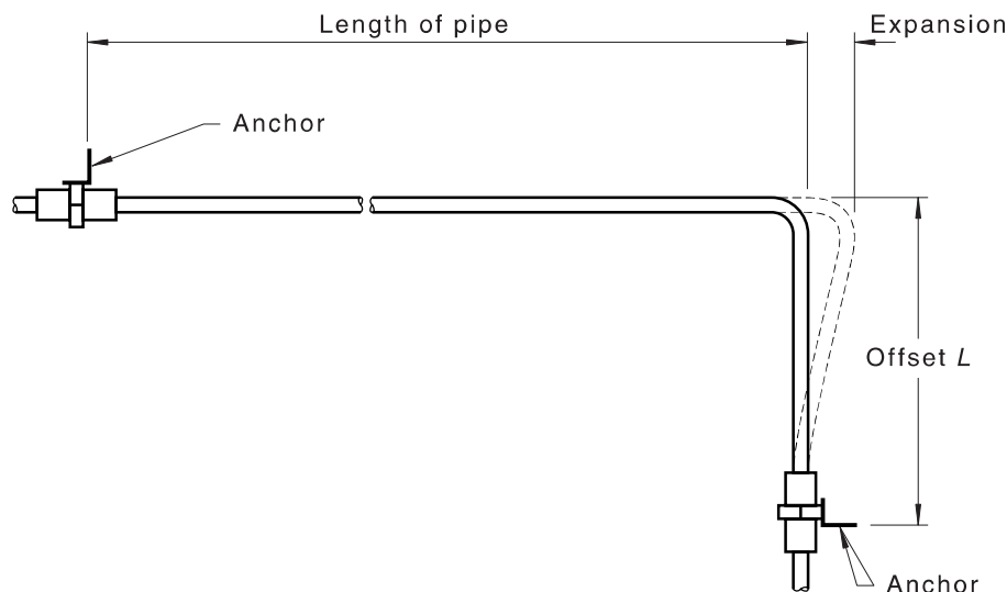
Figure N.4 — Offset to accommodate expansion
