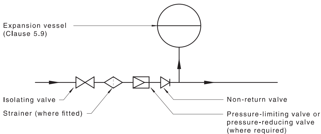
(b) Typical assembly with no pressure-limiting or pressure-reducing valve using an expansion vessel
