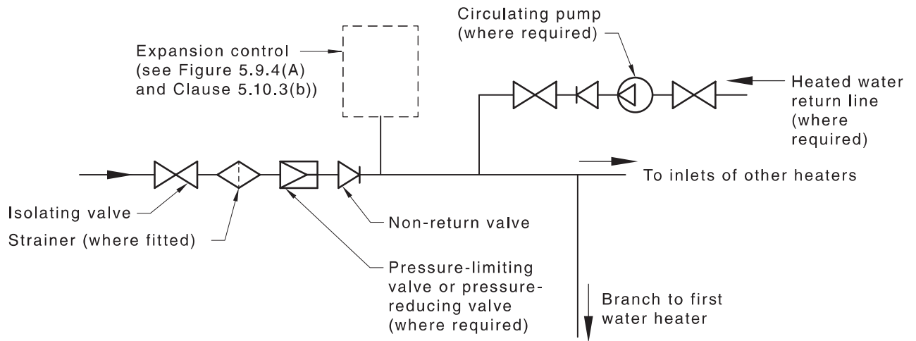
DETAIL A
