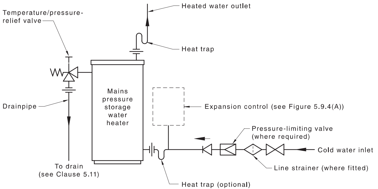
Figure 5.9.4(C) — Typical installation of a mains pressure storage water heater
