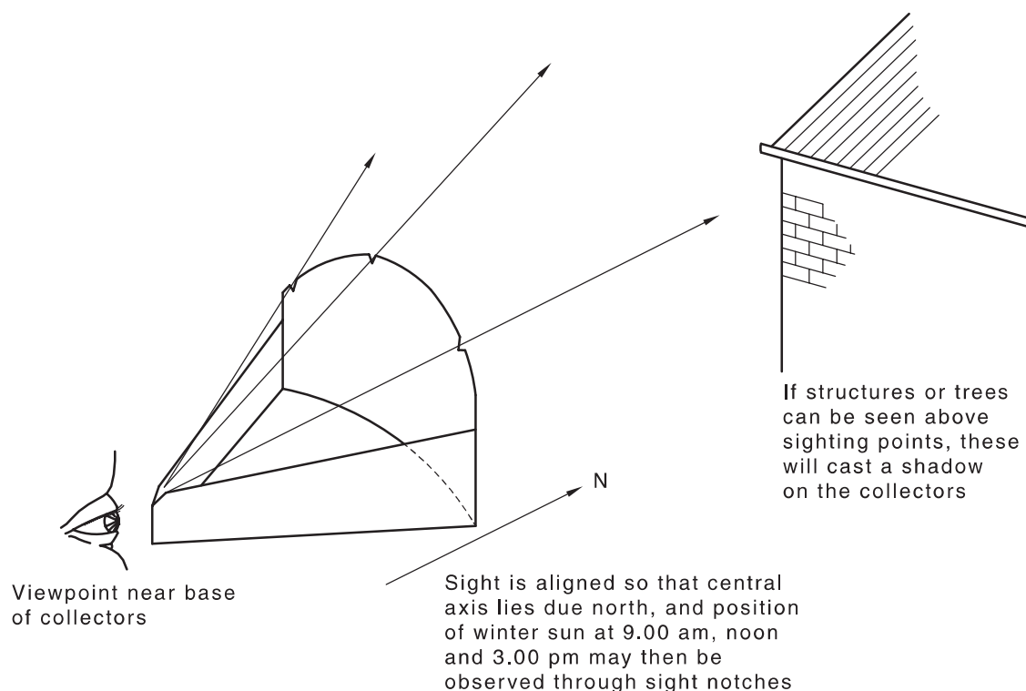
Figure H.2(C) — Use of solar altitude sight
