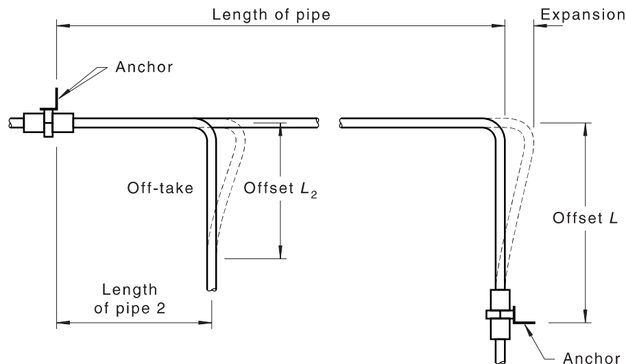
Figure N.9 — Expansion offset for branch off-take
