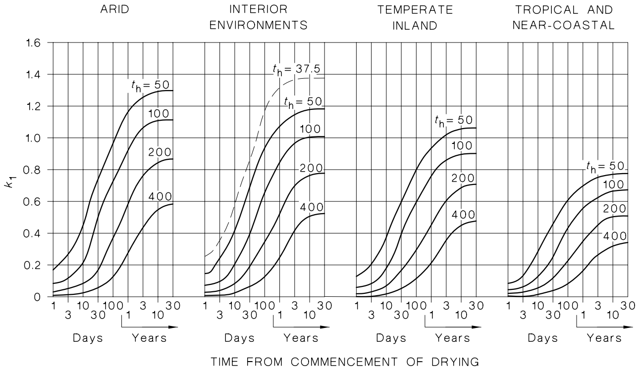
FIGURE 6.1.7.2 SHRINKAGE STRAIN COEFFICIENT ( k_1 ) FOR VARIOUS ENVIRONMENTS
