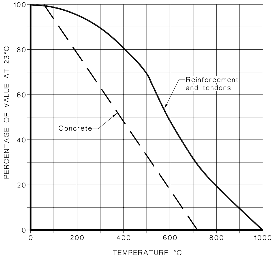
FIGURE 5.9(A) DECREASE OF ELASTIC MODULUS WITH TEMPERATURE
