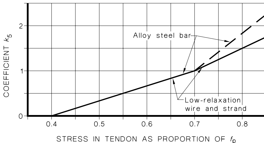
FIGURE 6.3.4.3 COEFFICIENT k_5
