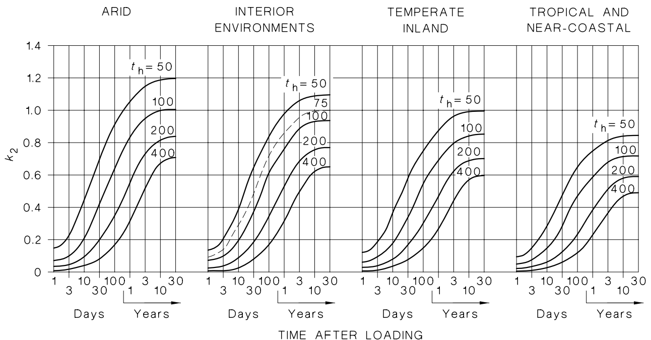
FIGURE 6.1.8.2 (A) CREEP FACTOR COEFFICIENT ( k_2 ) FOR VARIOUS ENVIRONMENTS
