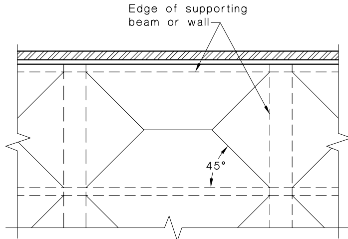
FIGURE 7.3.4 ALLOCATION OF LOAD
