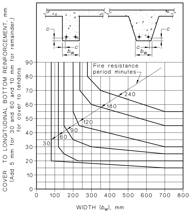
FIGURE 5.4.2(A) STRUCTURAL ADEQUACY REQUIREMENTS — SIMPLY SUPPORTED BEAMS
