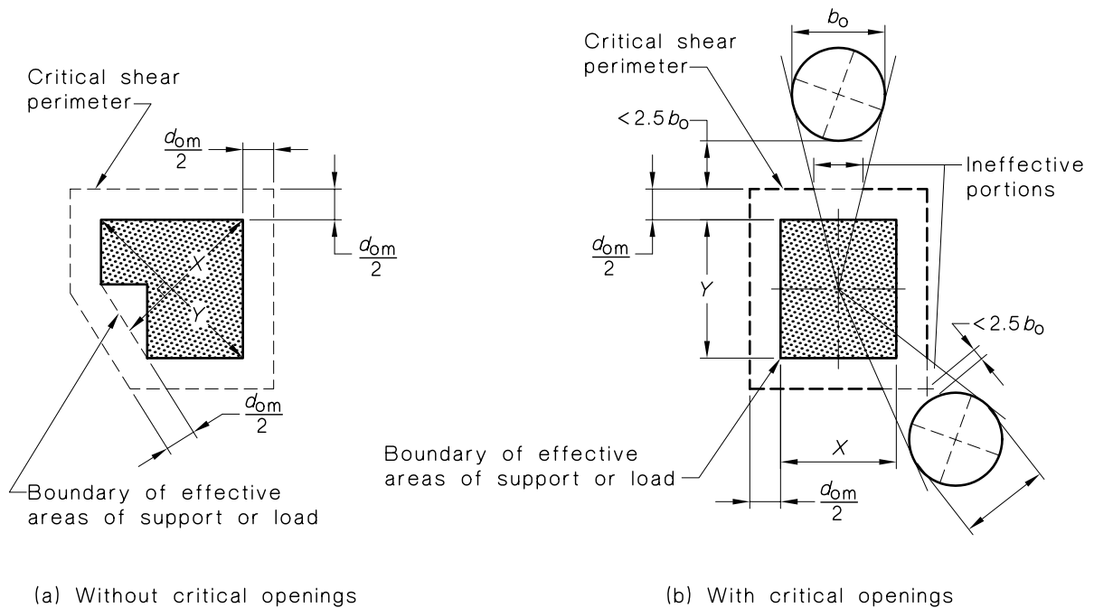
FIGURE 9.2.1(A) CRITICAL SHEAR PERIMETER
