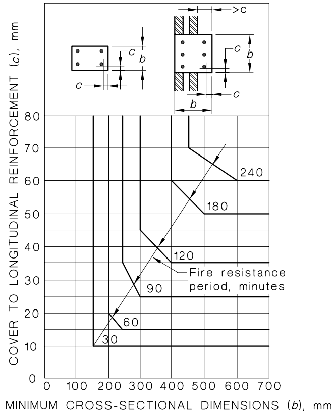
FIGURE 5.6.3 STRUCTURAL ADEQUACY REQUIREMENT — COLUMNS
