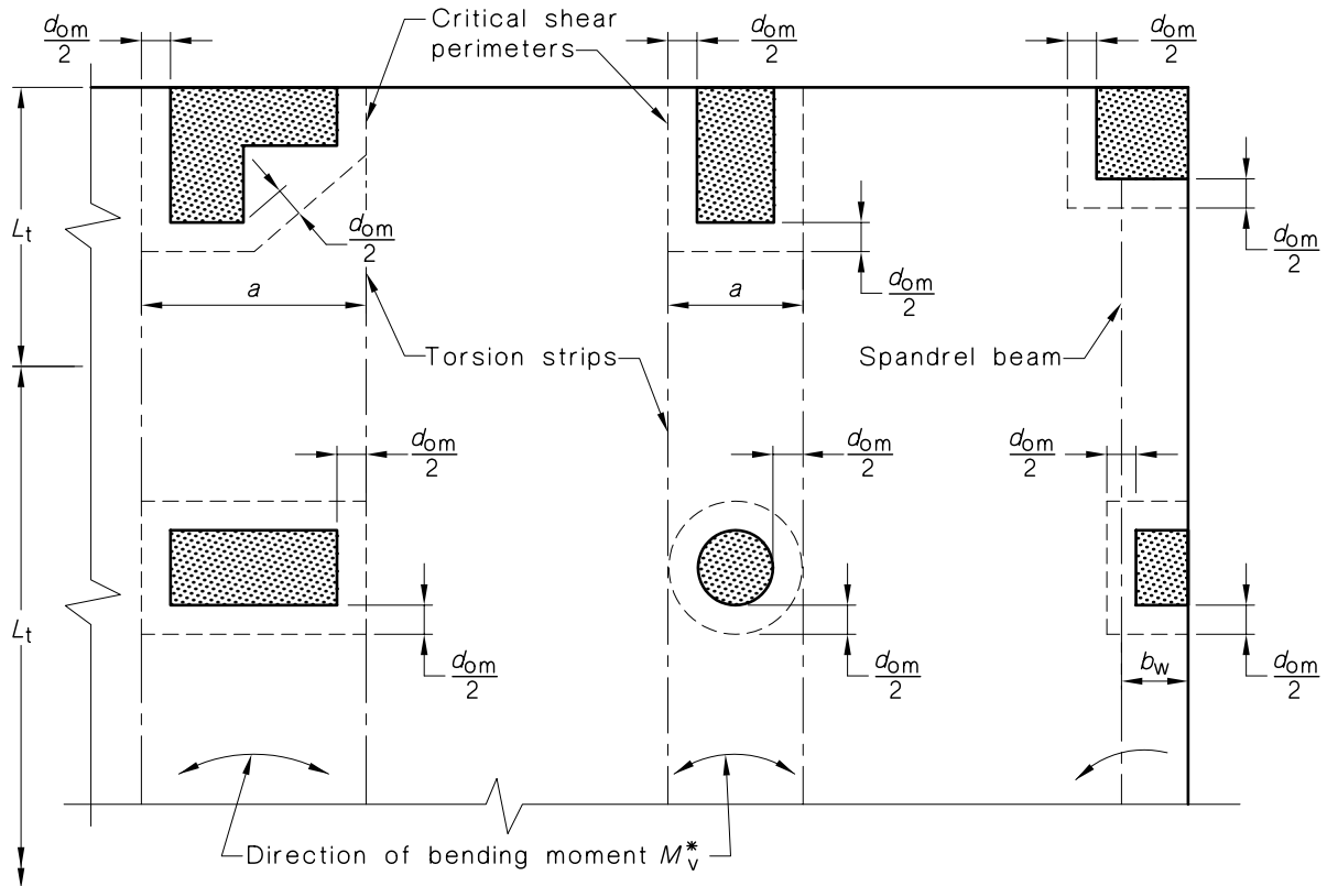
FIGURE 9.2.1(B) TORSION STRIPS AND SPANDREL BEAMS
