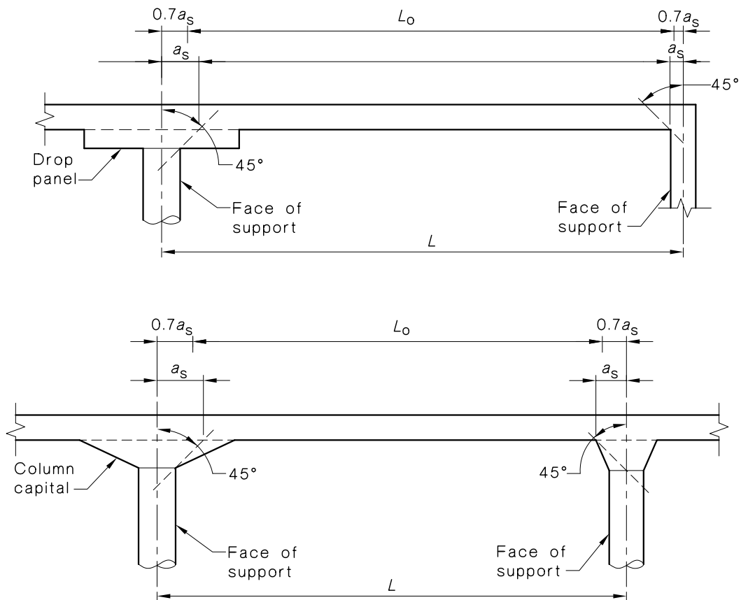
FIGURE 7.1.2(B) SPAN SUPPORT AND SPAN LENGTHS FOR FLAT SLABS
