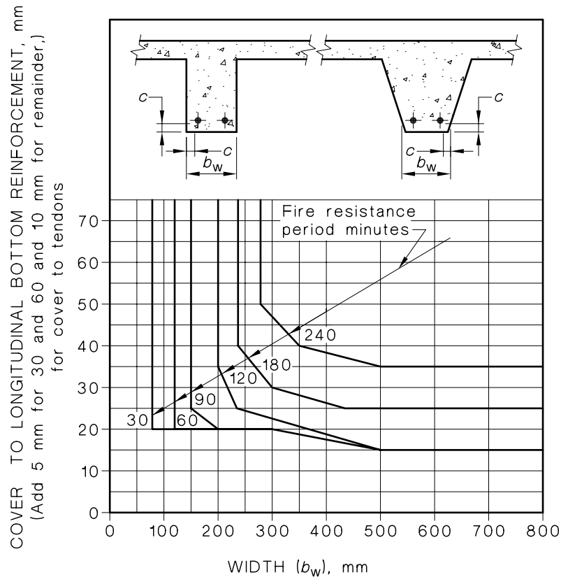
FIGURE 5.4.2(B) STRUCTURAL ADEQUACY REQUIREMENTS — CONTINUOUS BEAMS
