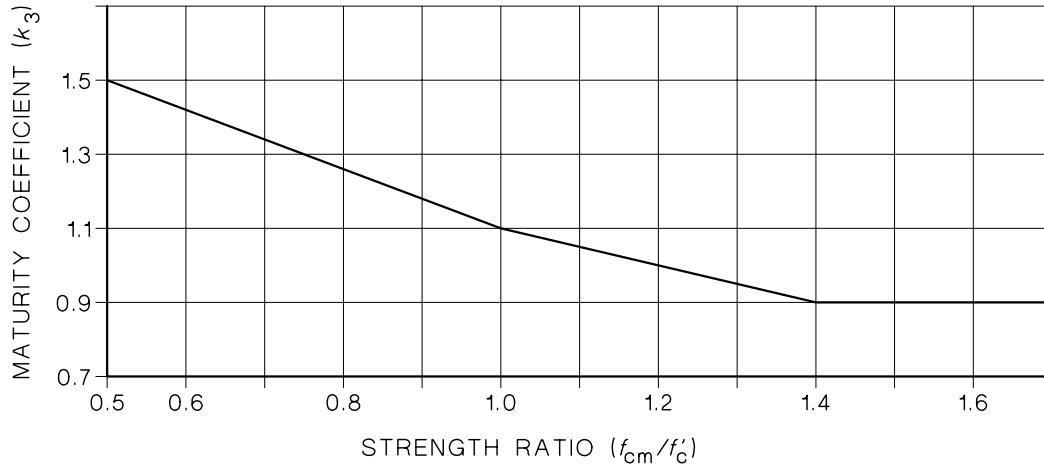
FIGURE 6.1.8.2(B) MATURITY COEFFICIENT ( k_3 )
