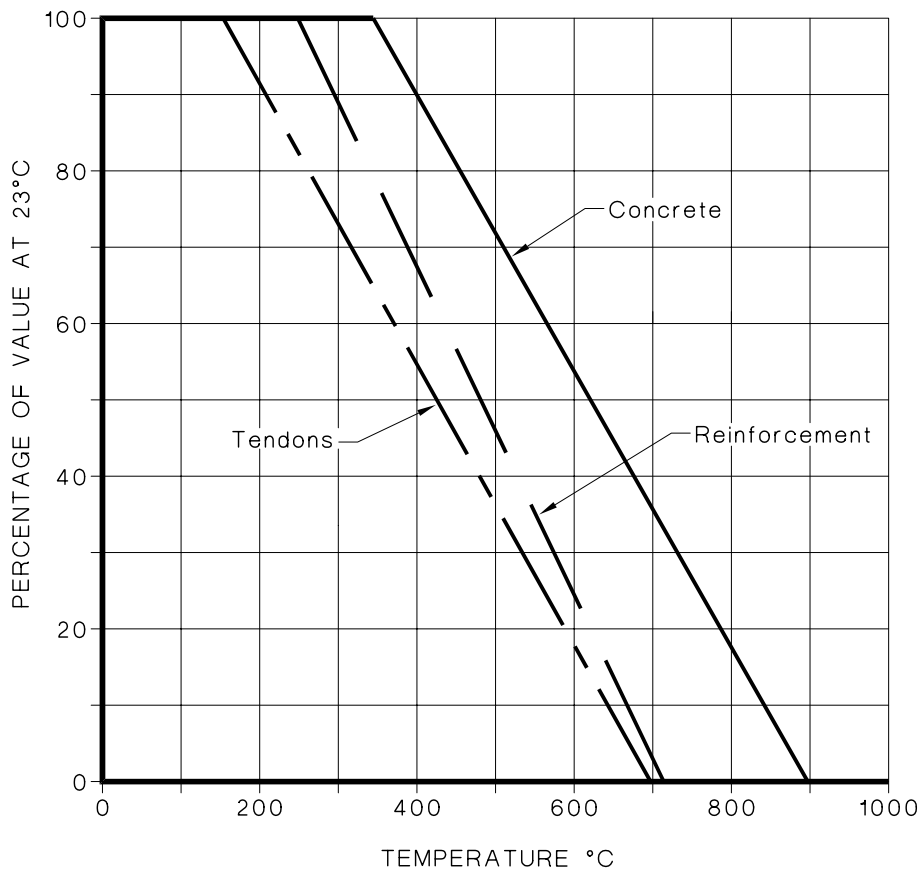
FIGURE 5.9(B) DECREASE OF STRENGTH WITH TEMPERATURE
