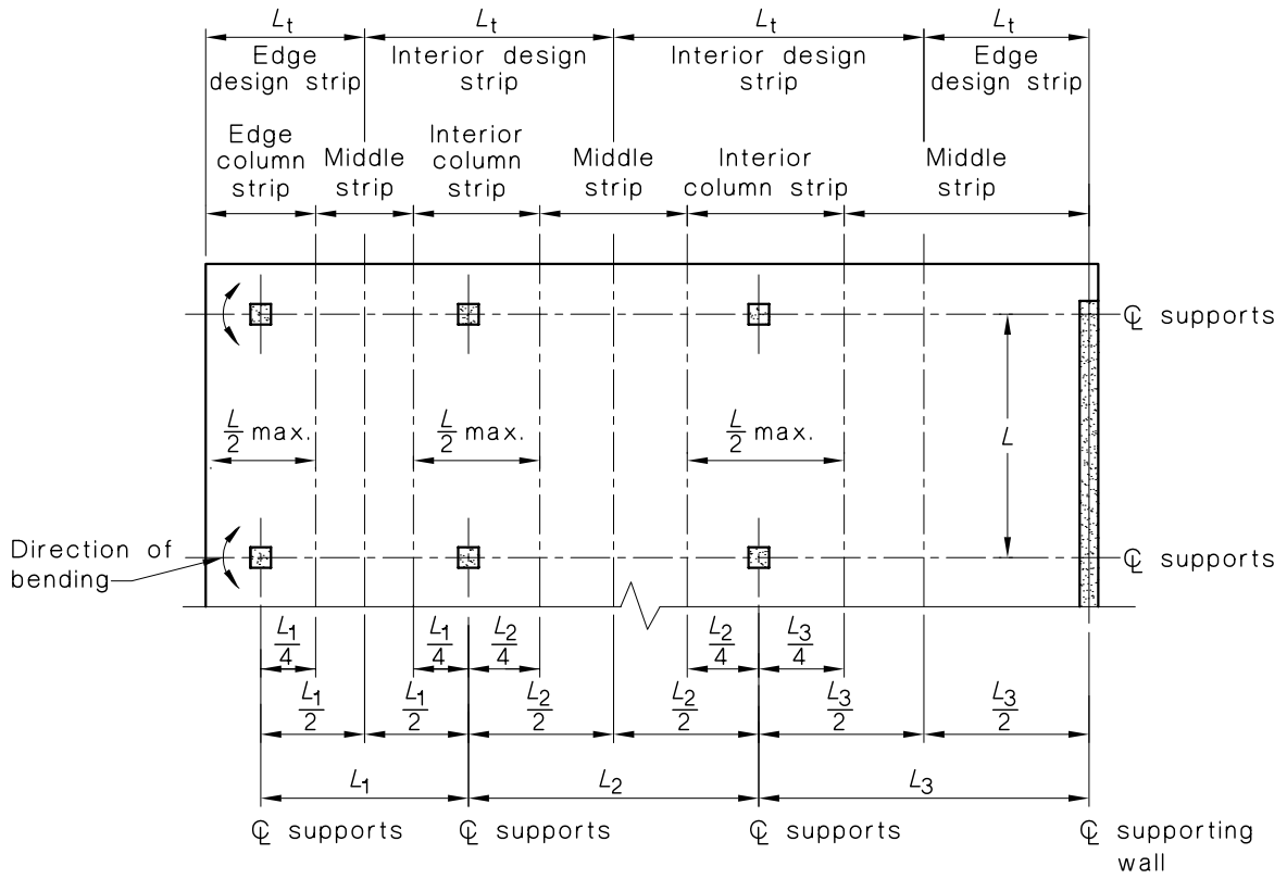
FIGURE 7.1.2(A) WIDTHS OF STRIPS FOR TWO-WAY SLAB SYSTEMS
