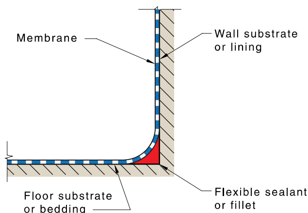
(b) Class III membrane
