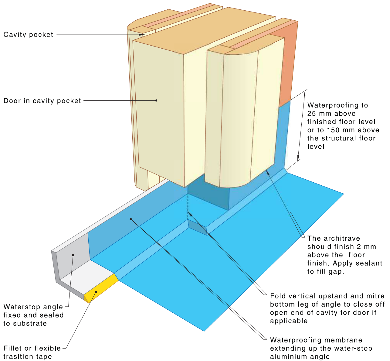
Figure 4.9.1(B) — Waterproofing at door opening cavity slider
