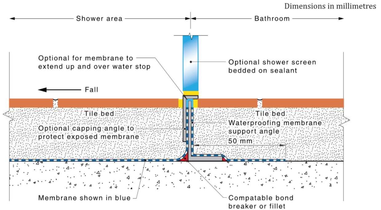
Figure 4.8.2(D) — Shower waterstop and cover angle
