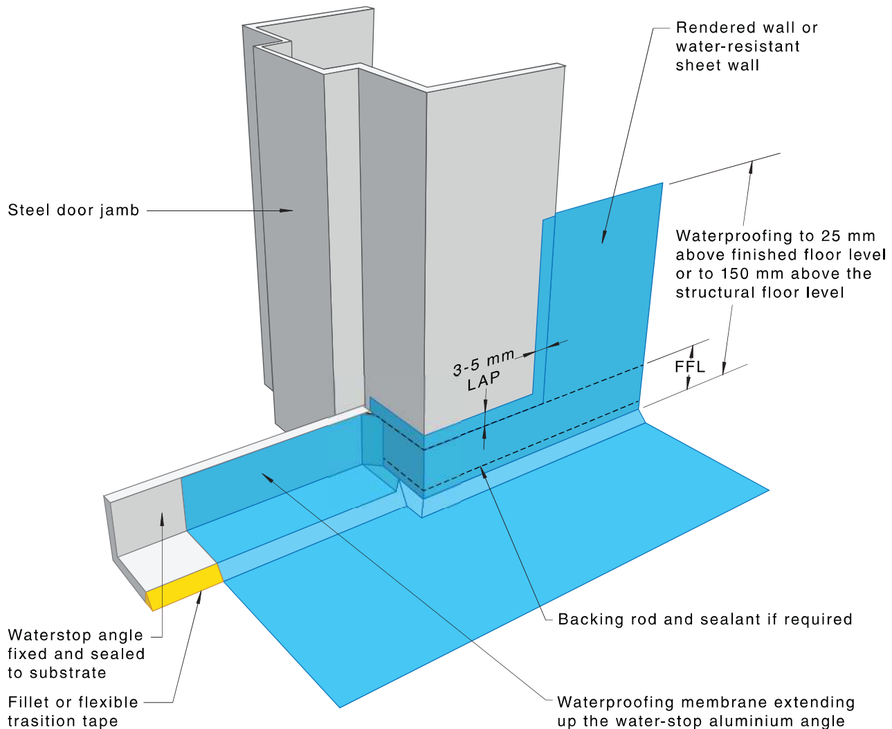
Figure 4.9.1(C) — Waterstop at door with steel frame
