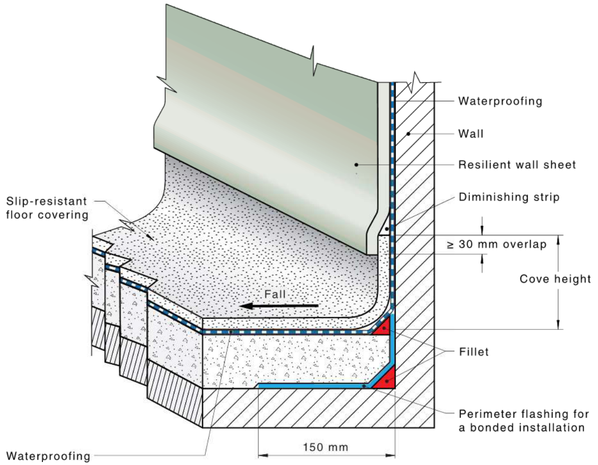
Figure 4.16(A) — Vinyl installation — Overlap method
