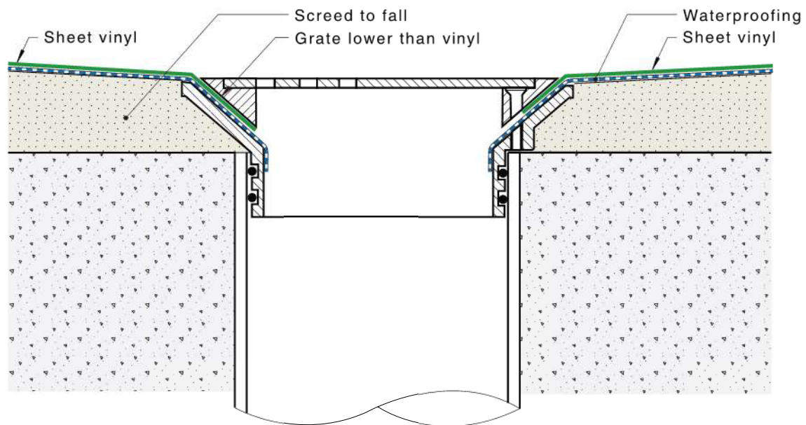
Figure 4.16(C) — Vinyl installation — Push-in vinyl sheet waste
