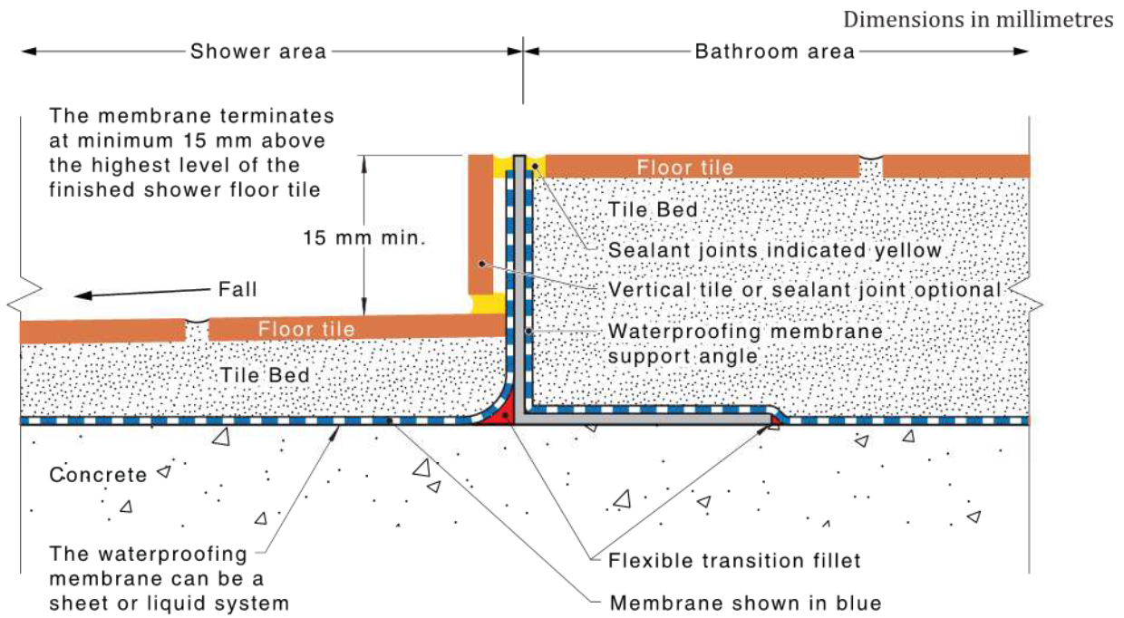
Figure 4.8.2(C) — Step-down shower waterstop and cover angle
