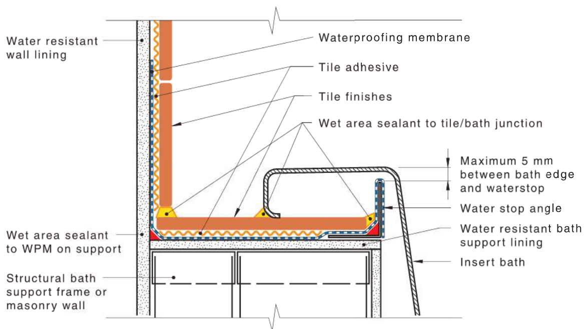
Figure 4.13.3(D) — Insert bath — Tile surround
