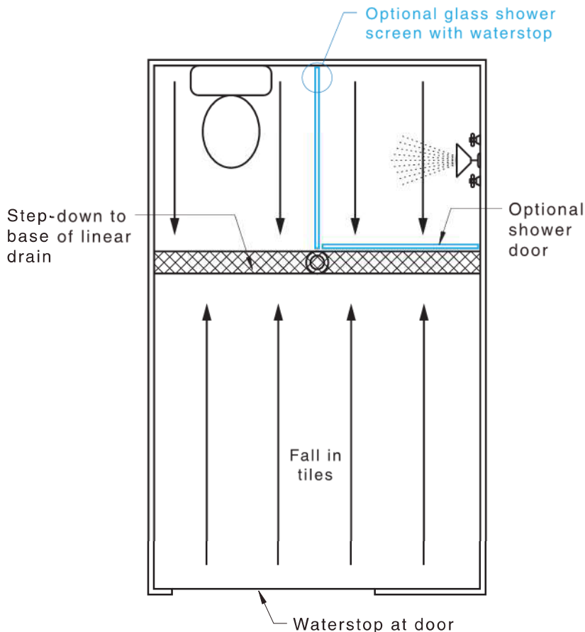
Figure A.6(A) — Whole of bathroom example
