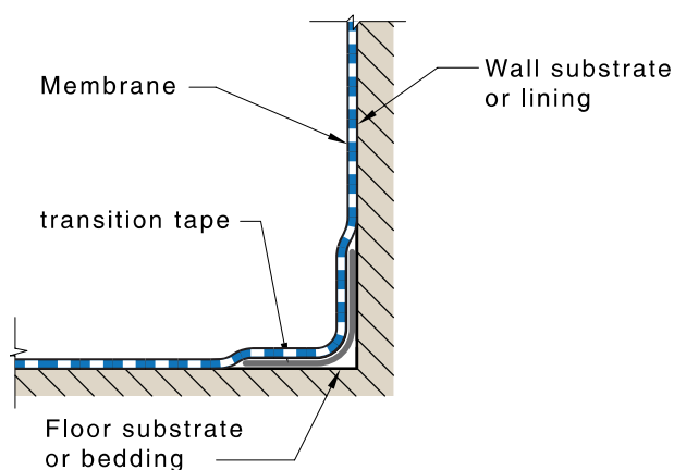
(a) Class I or II membrane
