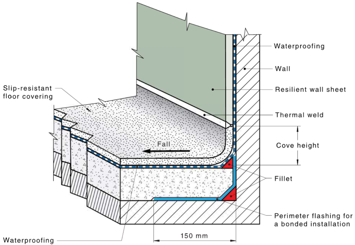
Figure 4.16(B) — Vinyl installation — Welded method
