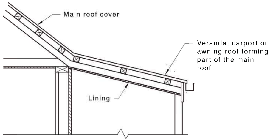
(a) Continuous roof
