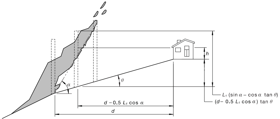
FIGURE B1 TYPICAL BUILDING AND FIRE FRONT CONFIGURATION
