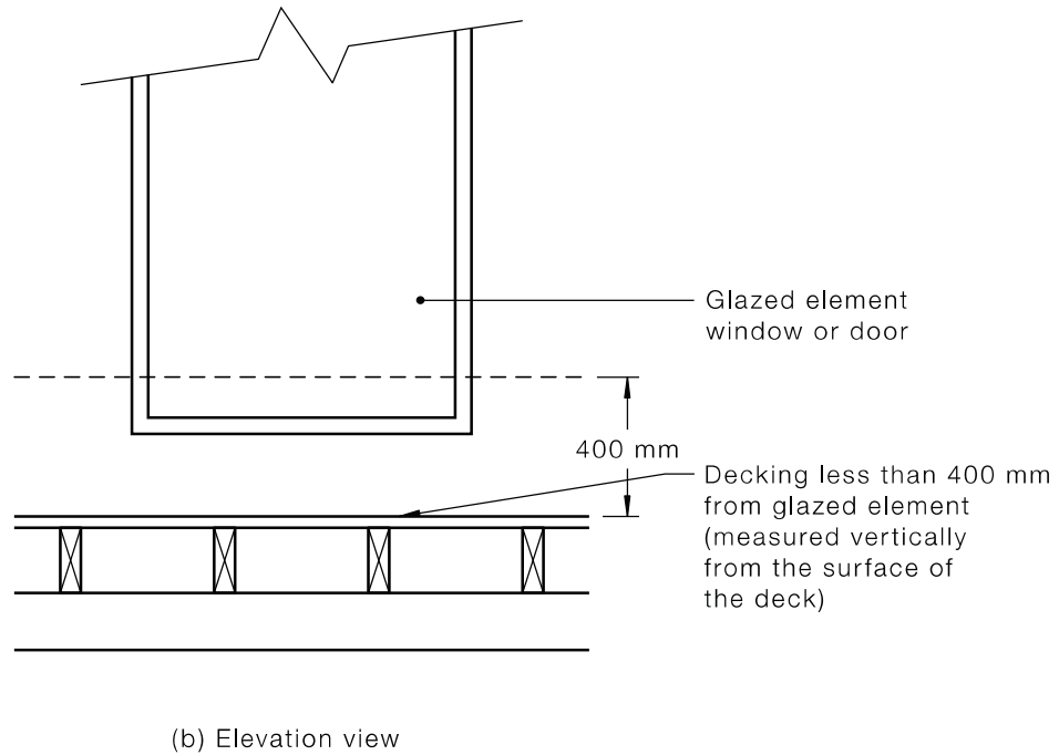
FIGURE D2 DECKING WITHIN HORIZONTAL AND VERTICAL LIMITS OF GLAZED ELEMENTS
