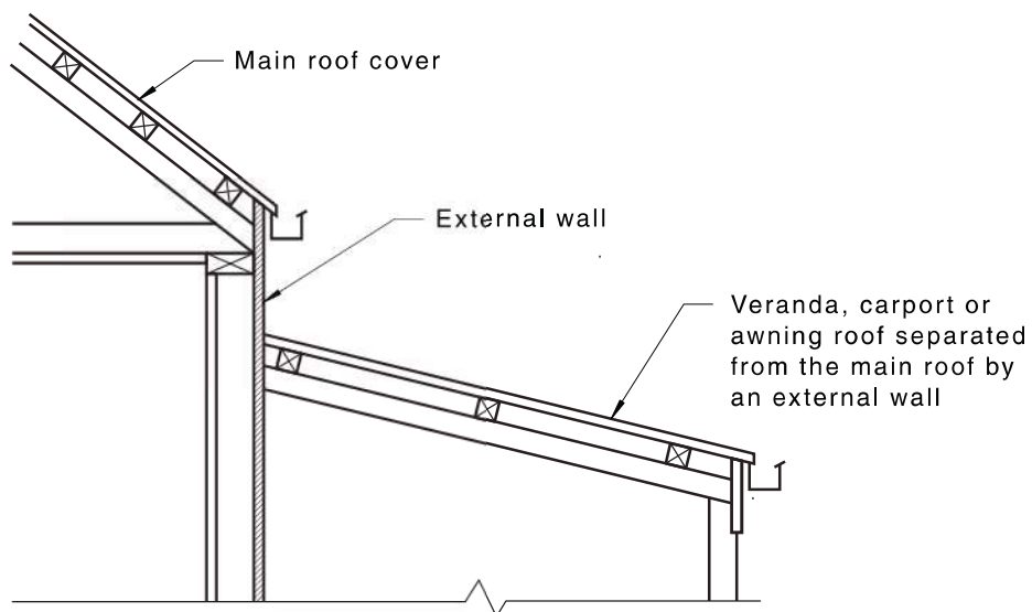
(c) Discontinuous roof
