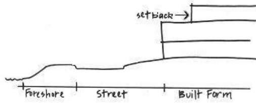
Figure CCO-S3.4 Building rhythm with alternating built and natural views as required by clause CCO-S3.7.2 P1(c)(iii)
