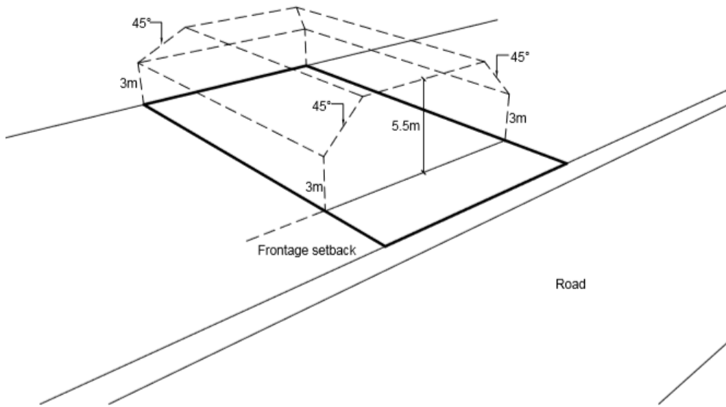
Figure CCO-S5.2 - Building envelope for corner lots as required by clause CCO-S5.7.1 A1 and A2 that is in substitution for General Residential Zone - clause 8.4.2 A3 and clause 8.5.1 A2
