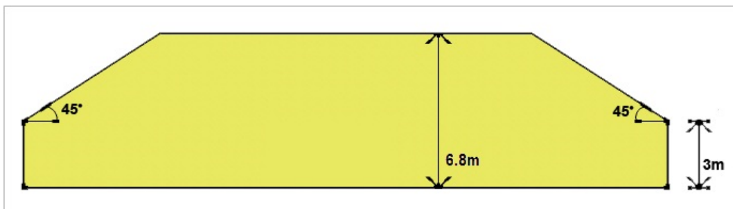
Figure DOR-P1.1 - Building envelope required by DOR-P1.6.3 A1(b)
