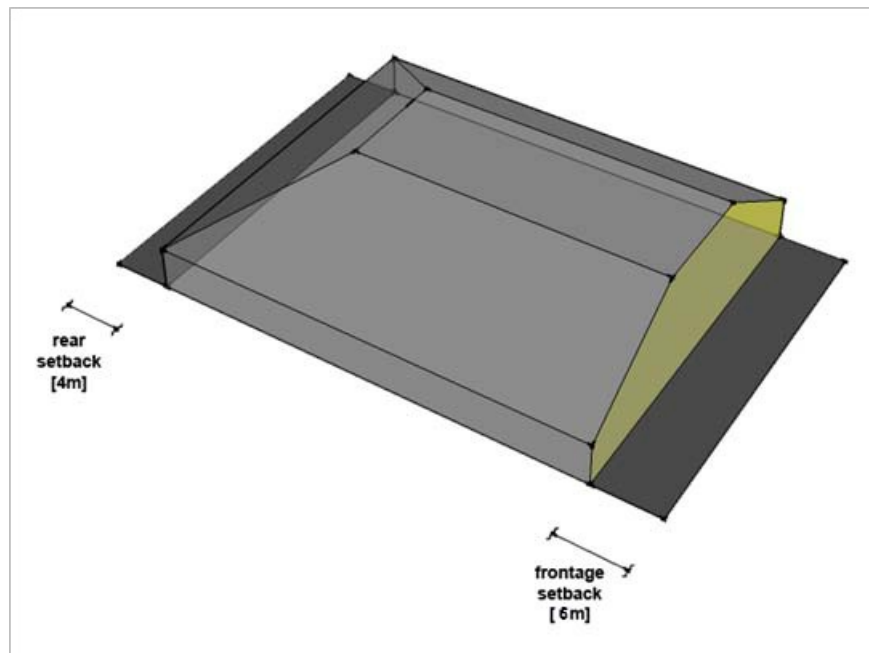
Figure DOR-P1.2 - Building envelope required by DOR-P1.6.3 A1(b)
